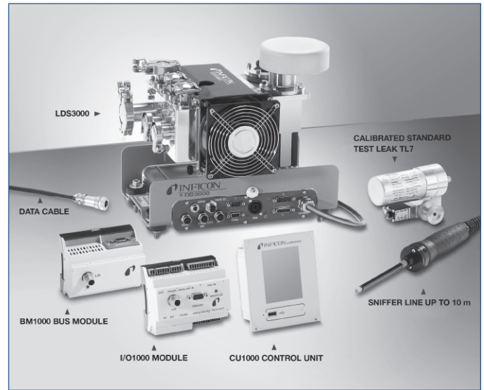
System schematics LDS3000
