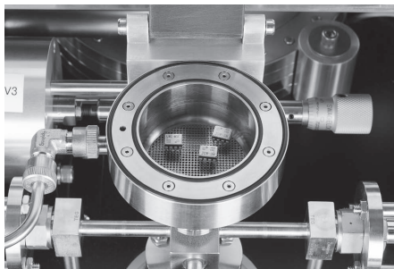
CHLD 700H probe chamber with test components
