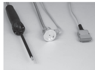
Helium sniffer line SL 200 P
